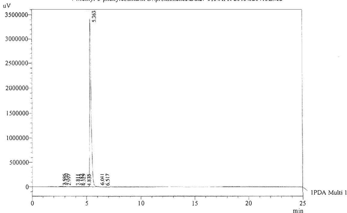
Chromatogram 4-Methyl-3-phenylcoumarin D:\promonence\Data\ 013\APR-2013\020413E.lcd
